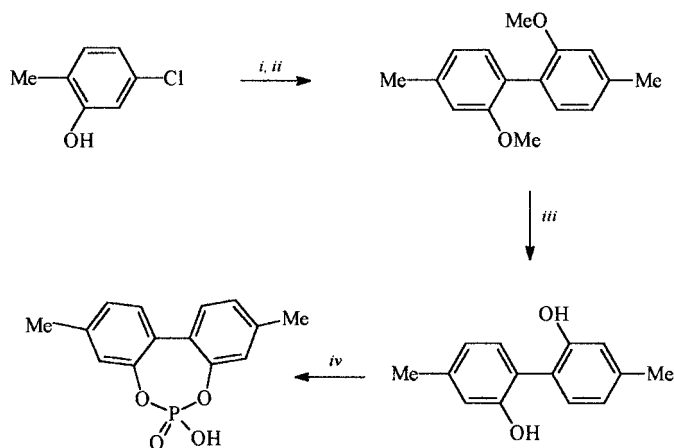
Scheme 2. Reagents: (i) \text{Me}_2\text{SO}_4 , NaOH; (ii) \text{NiCl}_2\text{ZnPPH}_3 , \alpha -dipy, DMF, 120^\circ\text{C} ; (iii) HBr/HOAc; (iv) polyphosphoric acid.
