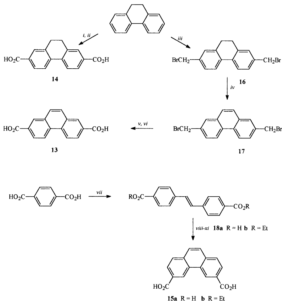
Scheme 1. Reagents: (i) \text{CH}_3\text{COCl} , \text{AlCl}_3 ; (ii) \text{I}_2 , pyridine then \text{NaOH}/\text{aq. EtOH} ; (iii) (\text{CH}_2\text{O})_n , \text{HBr} , \text{H}_3\text{PO}_4 in aq. \text{HOAc} ; (iv) DDQ, benzene; (v) DMSO, \text{NaHCO}_3 ; (vi) \text{bipyH}_2\text{CrOCl}_3 , \text{CH}_2\text{Cl}_2 ; (vii) S 270–275°C; (viii) \text{SOCl}_2 ; (ix) \text{EtOH} ; (x) h\nu , \text{I}_2 , \text{O}_2 , toluene; (xi) aq. \text{NaOH} .
